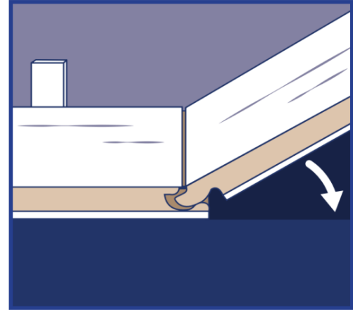
Step 2: Lock short end of plank by inserting tongue into groove at an angle and drop in place. Continue to end of first row.
